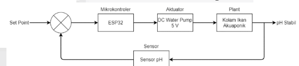
GAMBAR 3 Diagram Blok Sistem Kendali
