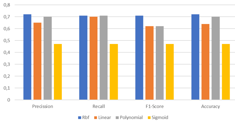
Gambar 16. Diagram Perbandingan Kernel Trick SVM (80/20)
