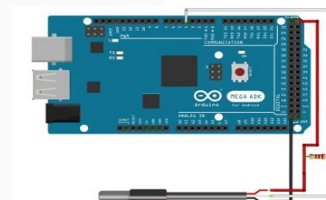
GAMBAR 2 wiring Sensor Suhu DS18B20
