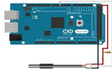
GAMBAR 3 wiring sensor Dissolved Oxygen DF robot
