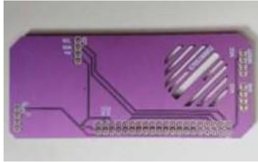
Gambar 16 Shield PCB
