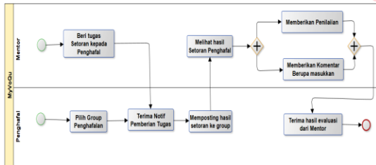
Gambar 5 Proses Bisnis Usulan Setoran Hafalan
