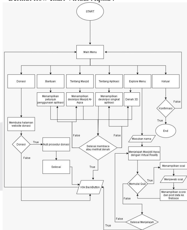
Gambar 2 Flowchart System
