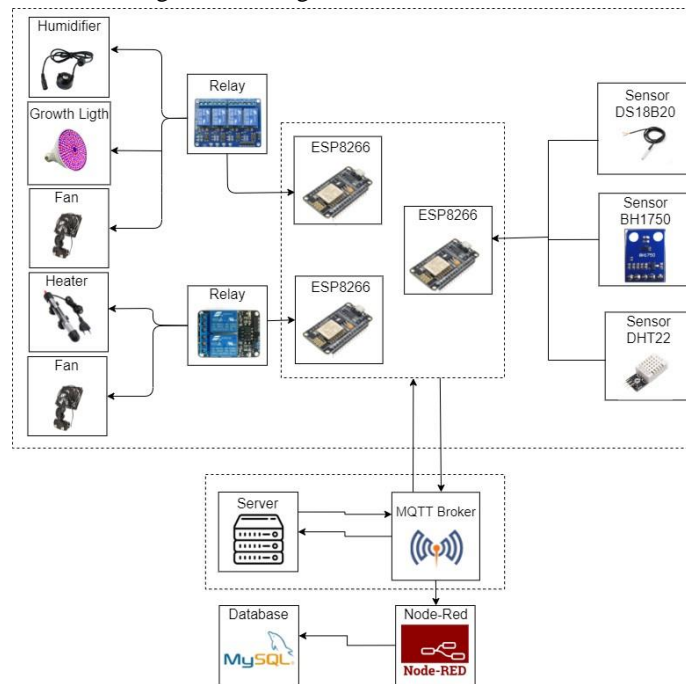
Figure 2. Block Diagram
