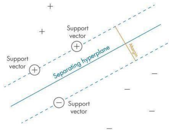
Picture 1. Support Vector Machine Architecture
