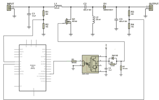
Gambar 3. 3 Wiring Diagram
