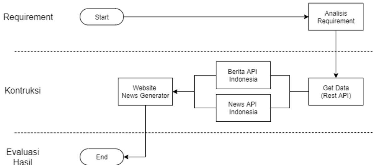
Gambar 4. Alur Penelitian
