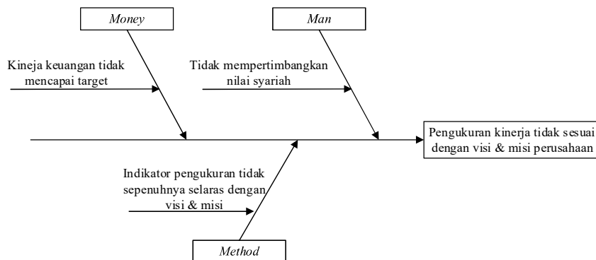
Gambar I-1 Fishbone Diagram
