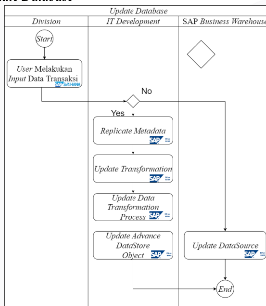
Gambar IV. 1 Proses Bisnis Update Database
