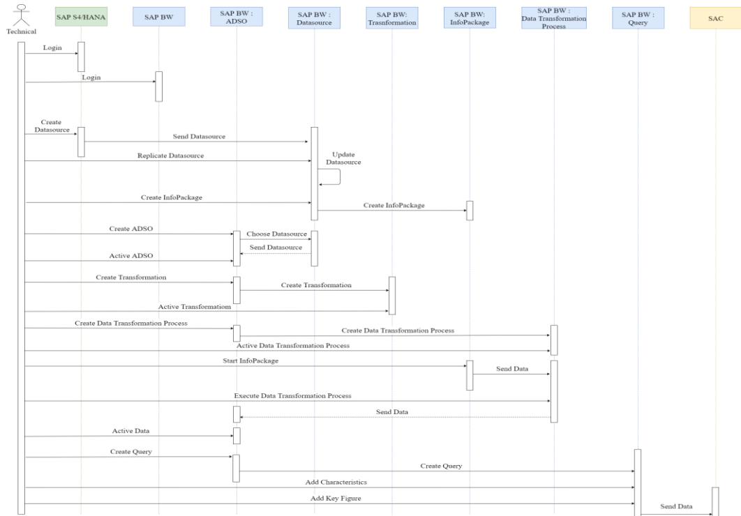
Gambar IV. 2 Sequence Diagram
