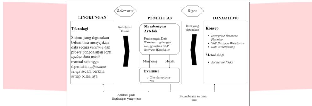
Gambar III.1 Model Konseptual
