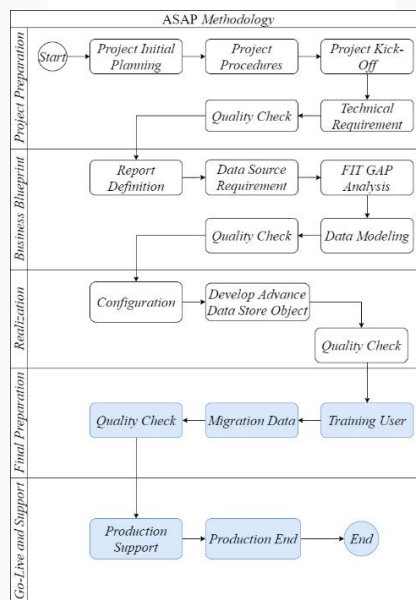
Gambar III.2 Sistematika Penelitian
