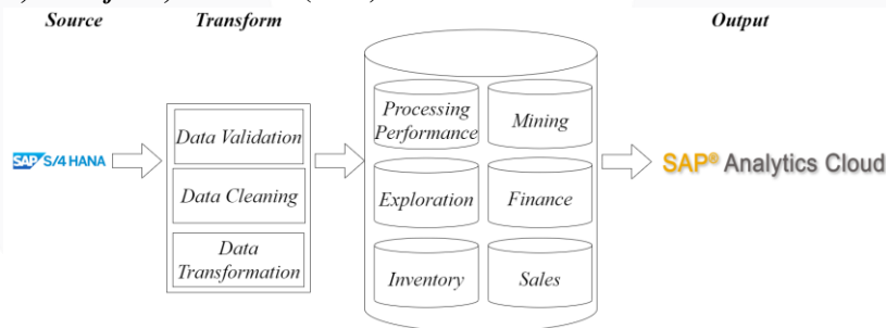
Gambar IV. 3 Extract, Transform, and Load
