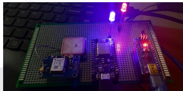
Gambar 4.13 Rangkaian Test.
