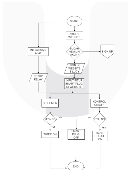
Gambar 3. 3 Diagram Alir Sistem Smart Plug
