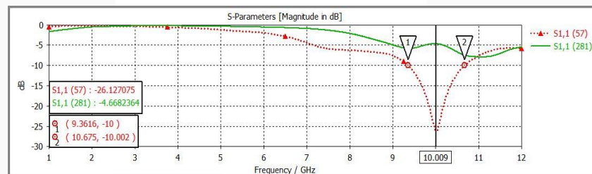
Fig. 5 - Returnloss Value of Antenna Model 2 Before and After Optimization.
