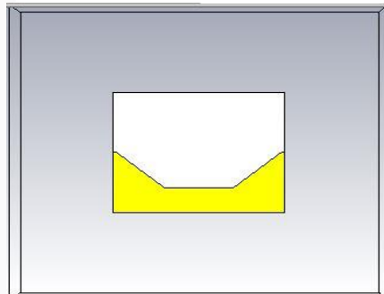
Fig. 1 – Structure of Trapezoidal-Cut Microstrip Antenna
