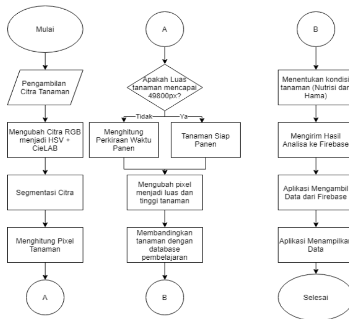
Gambar III-3. Flowchart Sistem.
