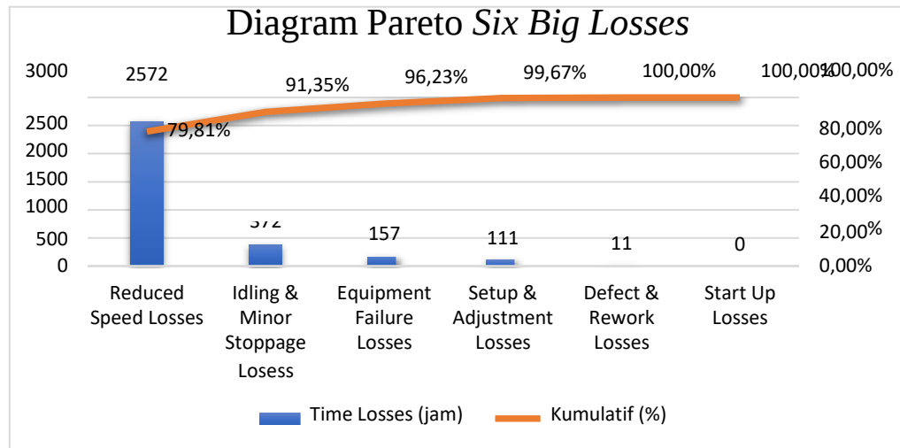
Gambar 4 Persentase Six Big Losses
