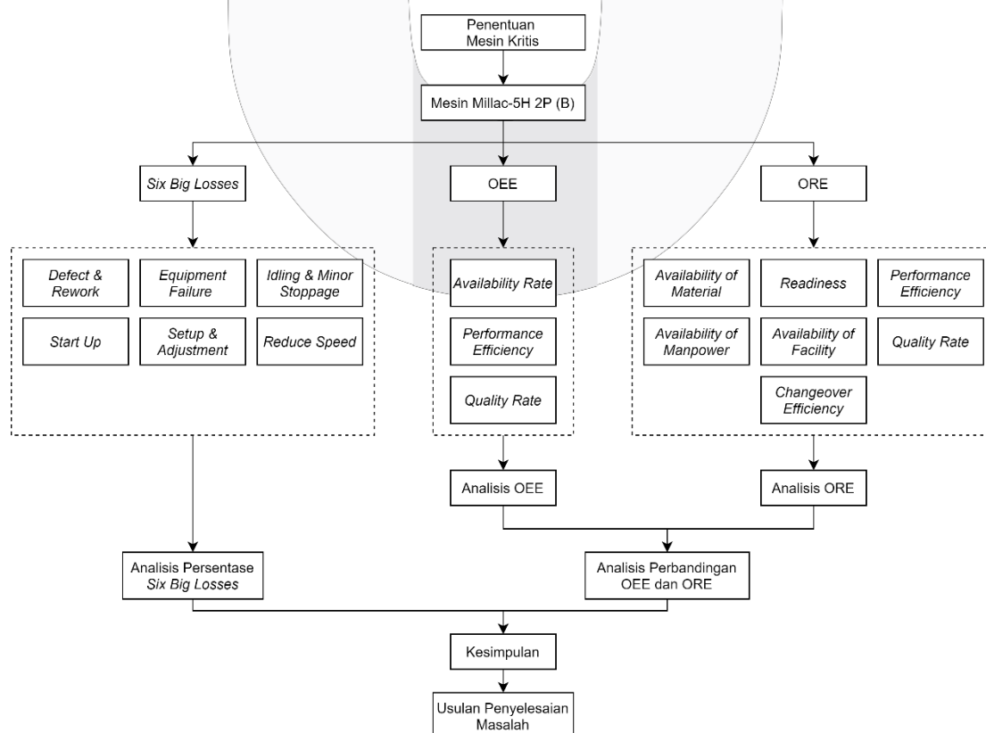
Gambar 2 Model Konseptual
