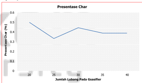
Gambar 6. Grafik Presentase Char
