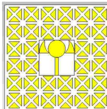
Figure 3.9 The Iteration 2 AMC Unit Cell
