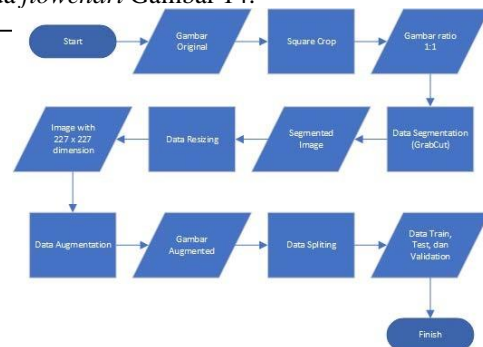
Gambar 14 Flowchart Preprocessing
