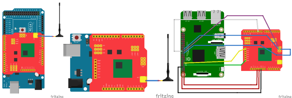
Gambar 3 Sketch Devices
