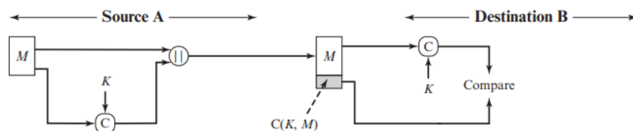
Gambar 1 Proses MAC [11, p. 389]
