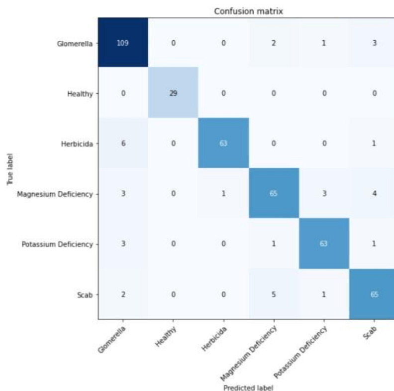
Gambar 7 Confusion Matrix
