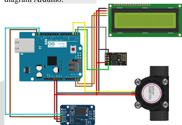
Gambar 4. 1 Rancangan Diagram Arduino
