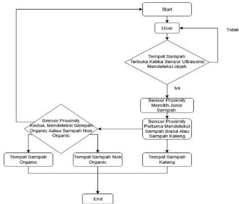
Gambar 3.2 Flowchart Hardware
