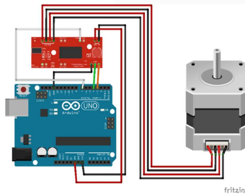
Figure 3.2 The figure shown the circuit of system
