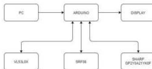
Figure 3.1 System Block How Arduino Connect With Other Sensors
