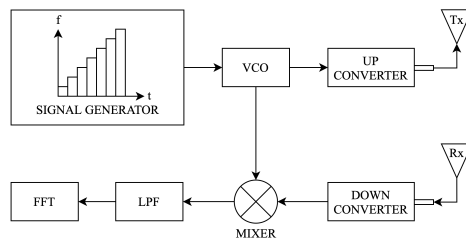
Gambar 3.1 Blok diagram radar SFCW.
