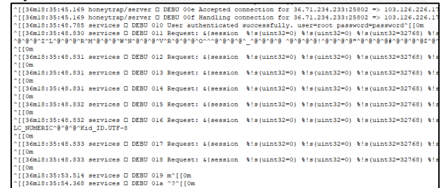
Gambar 4.11 Logs Serangan SSH
