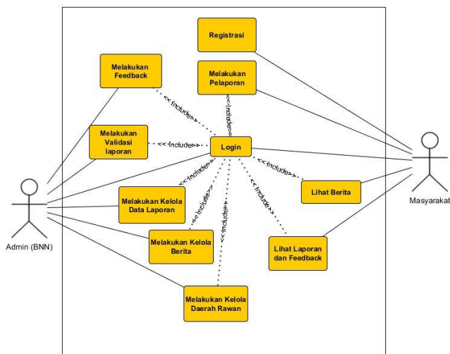
Gambar 2-2 Usecase
