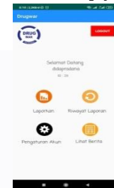
Gambar 2-6 Tampilan Dashboard
