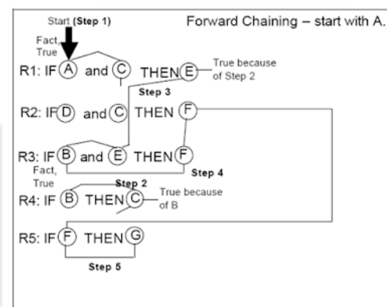
Gambar 2 Metode Forward Chaining
