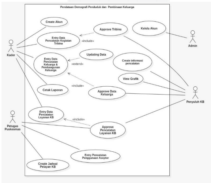
Gambar 4.3 Use Case
