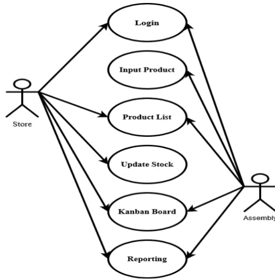
Gambar IV. 4 Use Case Diagram
