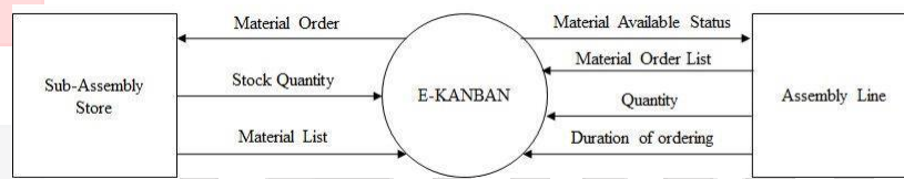
Gambar IV. 5 Data Flow Diagram
