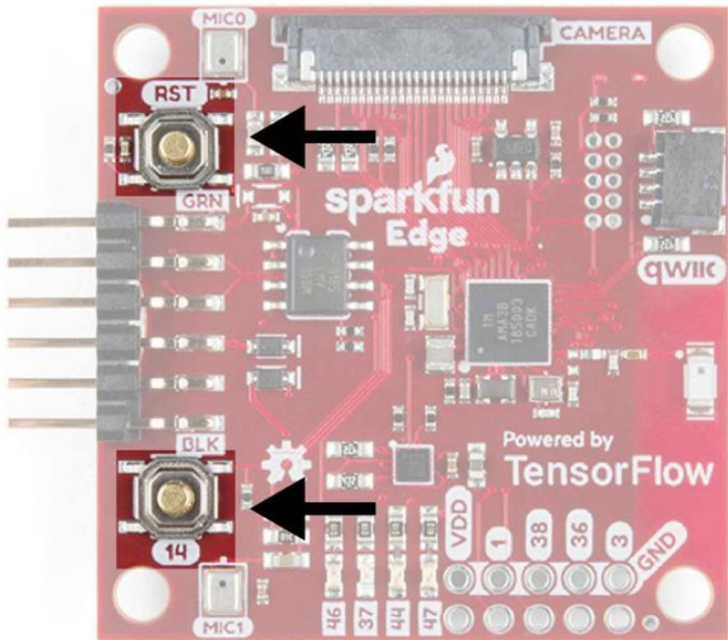
Figure 11-12. The SparkFun Edge's buttons
