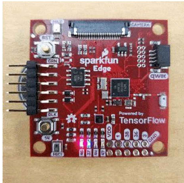
Figure 4-2. The code running on a SparkFun Edge
