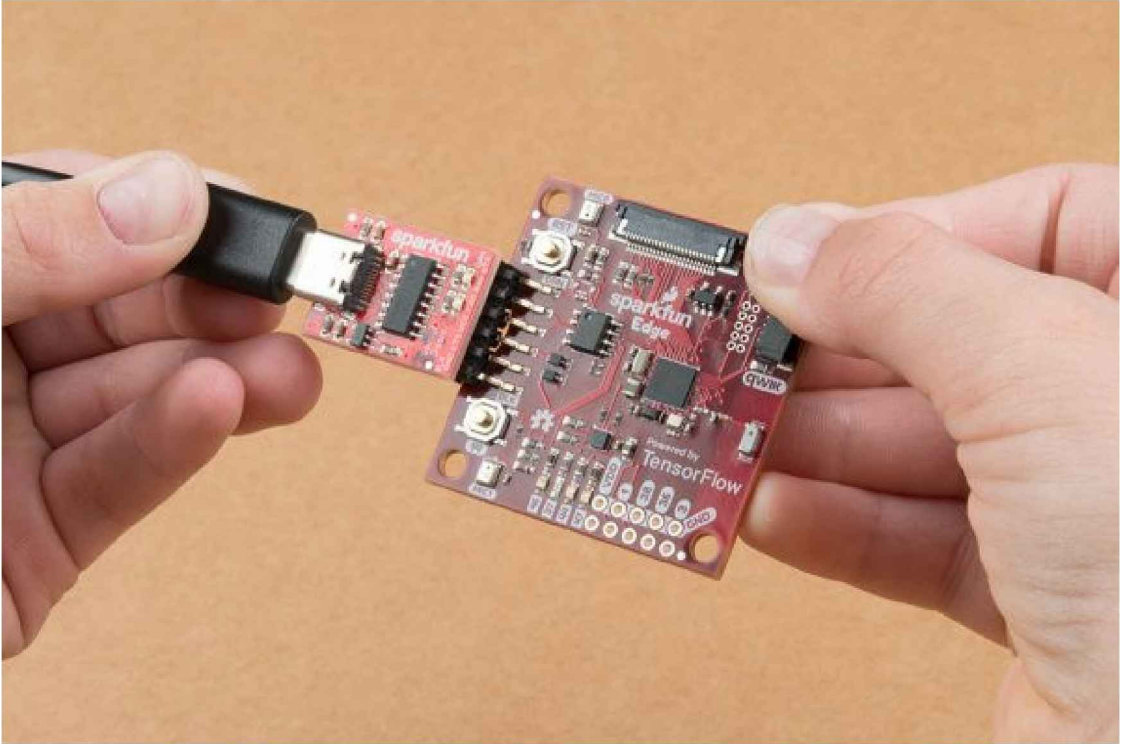
Figure 11-11. Connecting the SparkFun Edge and USB-C Serial Basic (image courtesy of SparkFun)
