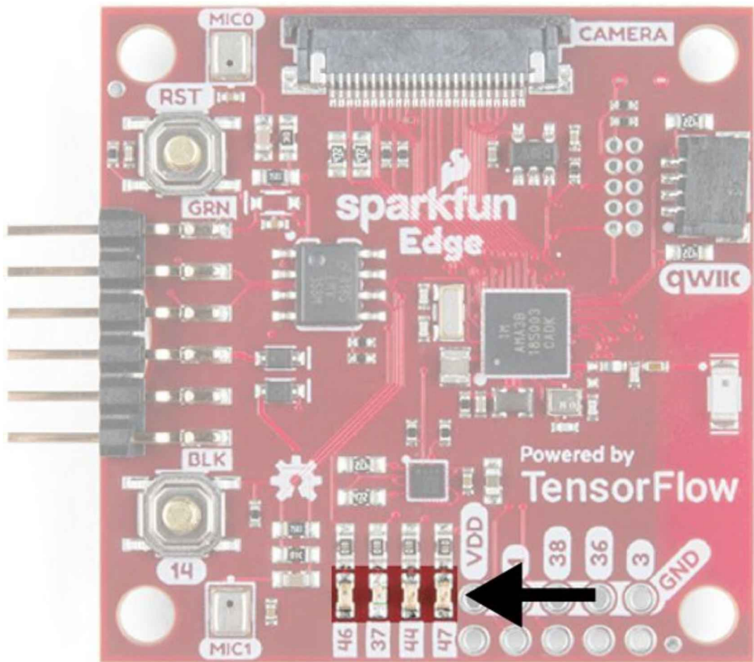
Figure 7-13. The SparkFun Edge's four LEDs
