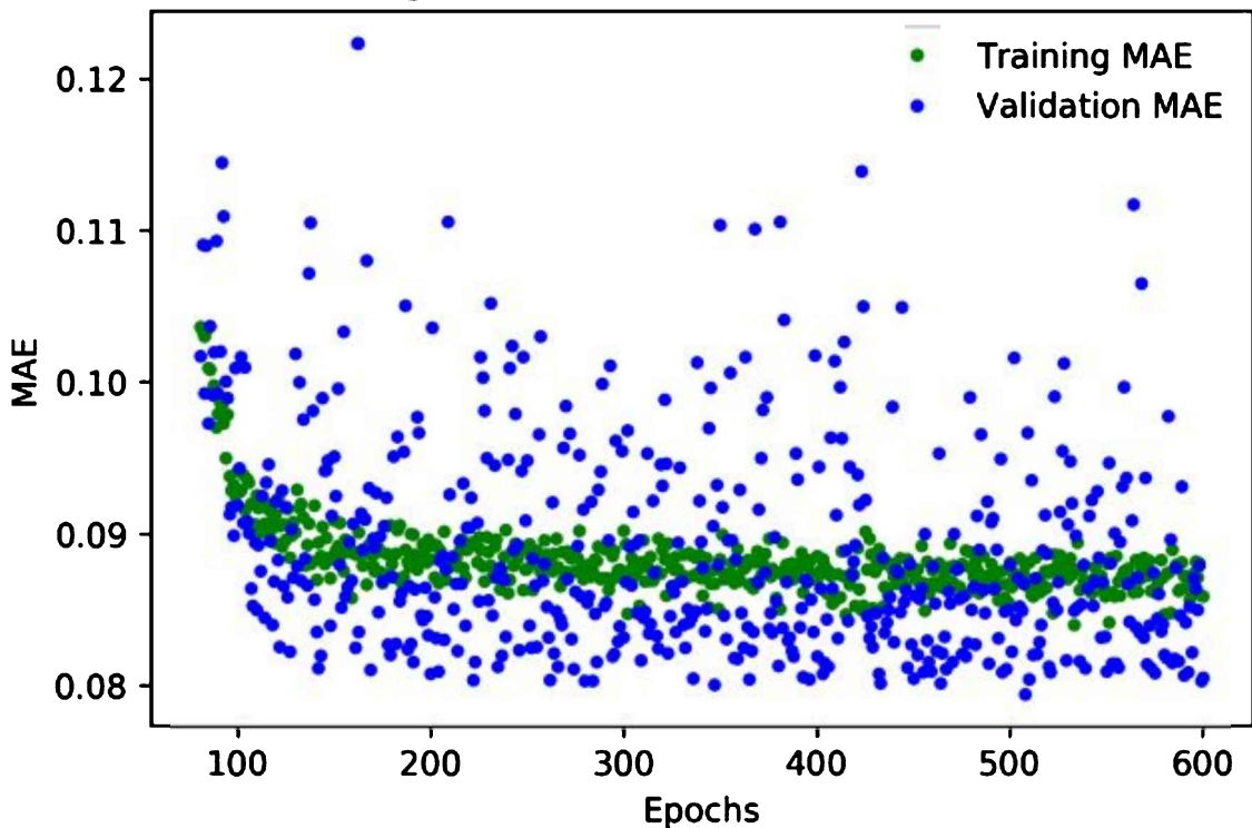
Figure 4-19. A graph of mean absolute error during training and validation
