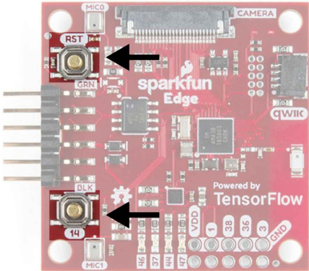
Figure 7-15. The SparkFun Edge's buttons
