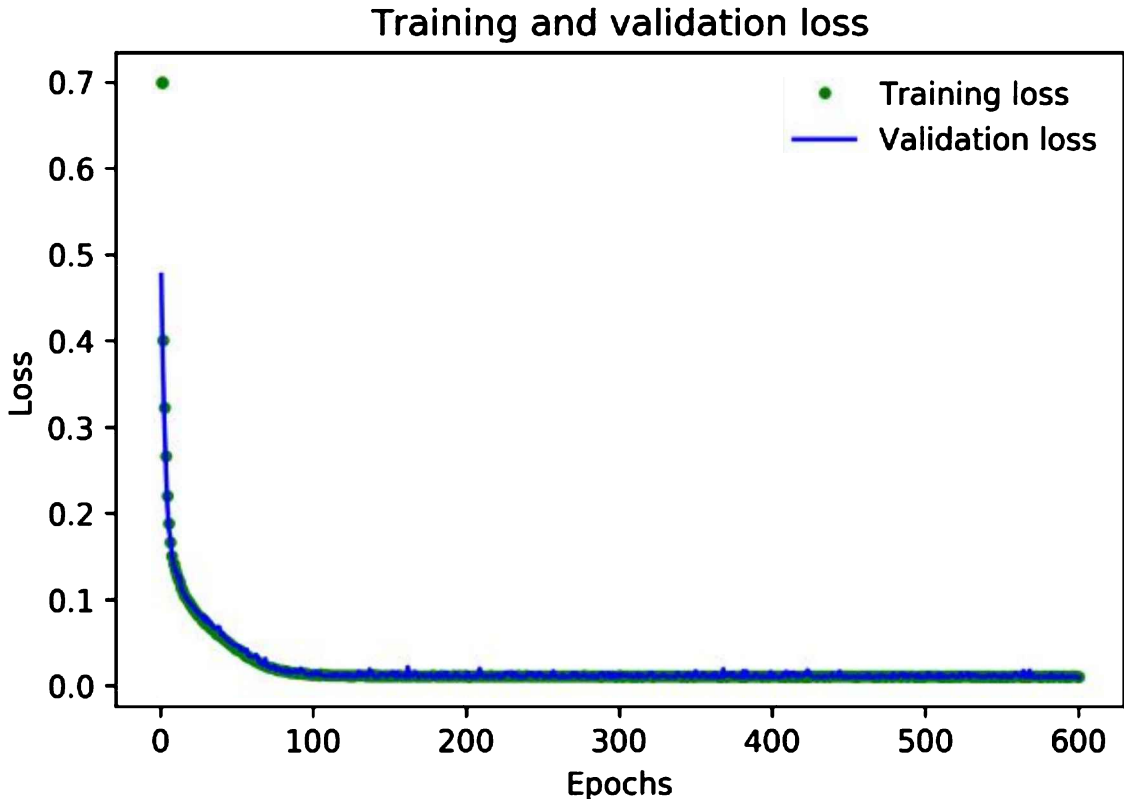
Figure 4-17. A graph of training and validation loss
