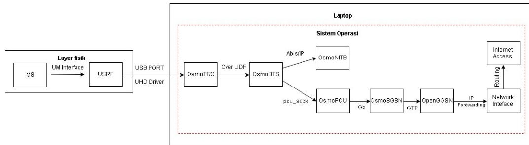
Gambar 2. Block Sistem
