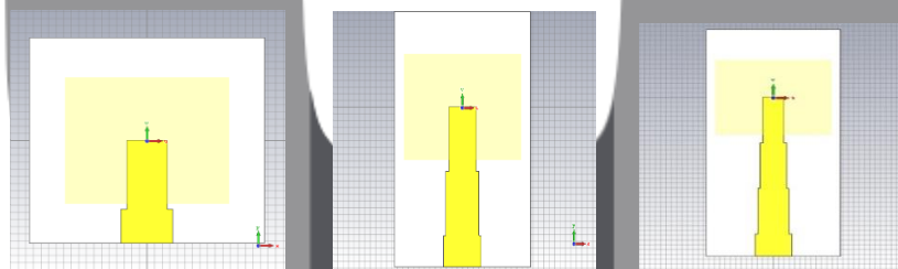
Gambar 3.1 Feed Line 1, 2, dan 3 Section.
