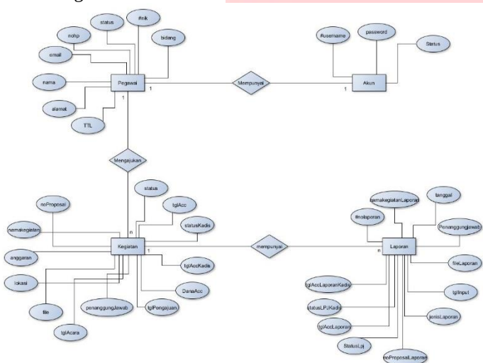
Gambar 8 Entity Relationship Diagram
