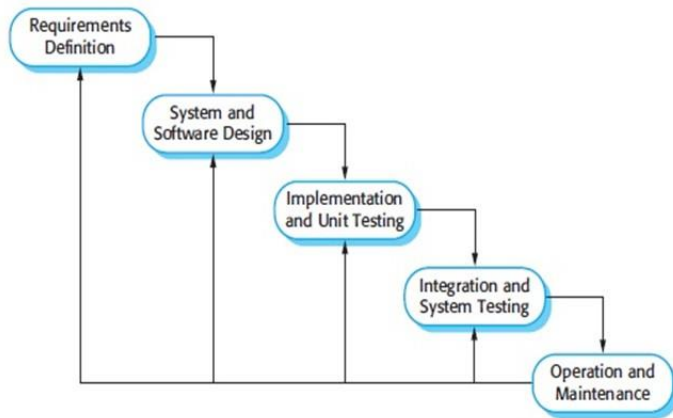
Gambar 1 Metode Waterfall [1]
