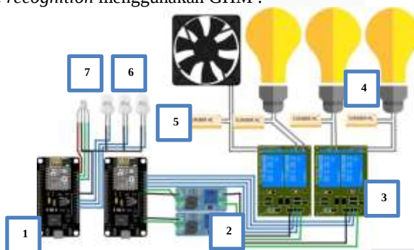
Gambar 3. 10 Perancangan Hardware
