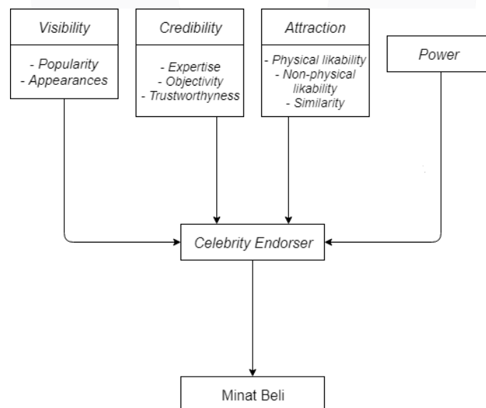
Gambar 3.1 Model Konseptual
