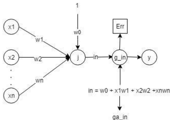
Gambar 1. Model Perceptron
