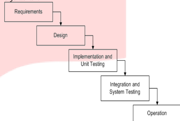
Gambar 3-1 Model Waterfall [2]
