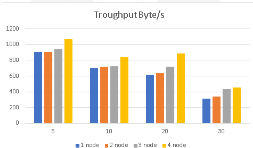
Gambar 8 Pengujian Throughput
