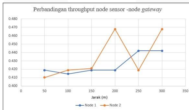
Gambar 6 Grafik Perbandingan Throughput Node Sensor – Node Gateway
