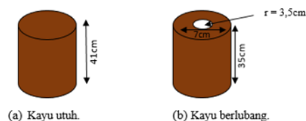
Gambar 2. Model objek.
