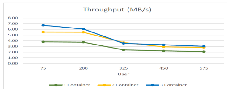
Gambar 4.2 Hasil throughput (MB/s)
