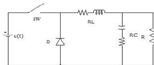
Gambar 2.2 Buck Converter
