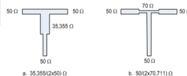
Gambar 4 T- Junction 50 ohm
