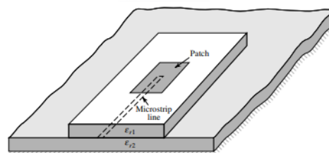
Gambar 2 Proximity coupled feeding
