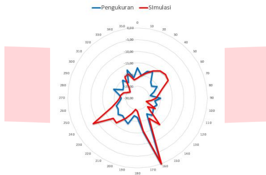
Gambar 16 Axial ratio pengukuran antenna
