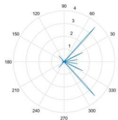
Gambar 13. Hasil Beamforming Antena 8 Elemen Jarak Lambda
