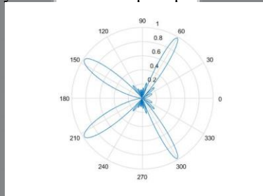
Gambar 10. Hasil Beamforming Antena Isotropis Jarak \frac{3}{4} Lambda
