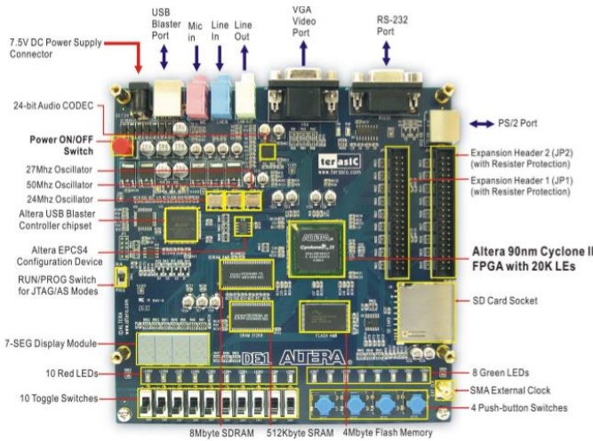
Gambar 3. DE1 Altera Board
