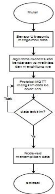
Gambar 3. Alur Diagram Sistem
