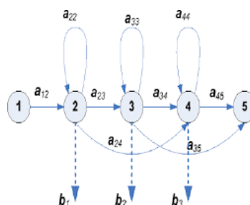
Gambar 3.3 State HMM
